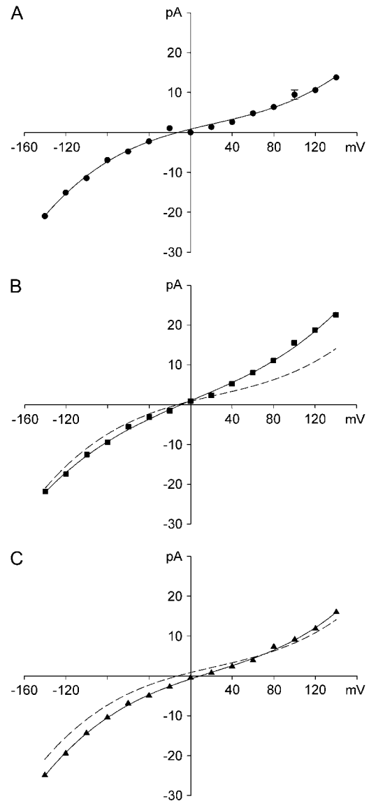
FIGURE 4 The current-voltage curves obtained using three different sets of the force constants. The force constants used for panels A, B, and C correspond to those used to construct Fig. 2 A. Each data point represents the average of 24 to 32 sets of simulations, each lasting 2 \times 10^6 time steps (or 0.2 \mu s ). Error bars in this and following figures have a length of mean \pm 1 SE and are not shown when they are smaller than the data points.
